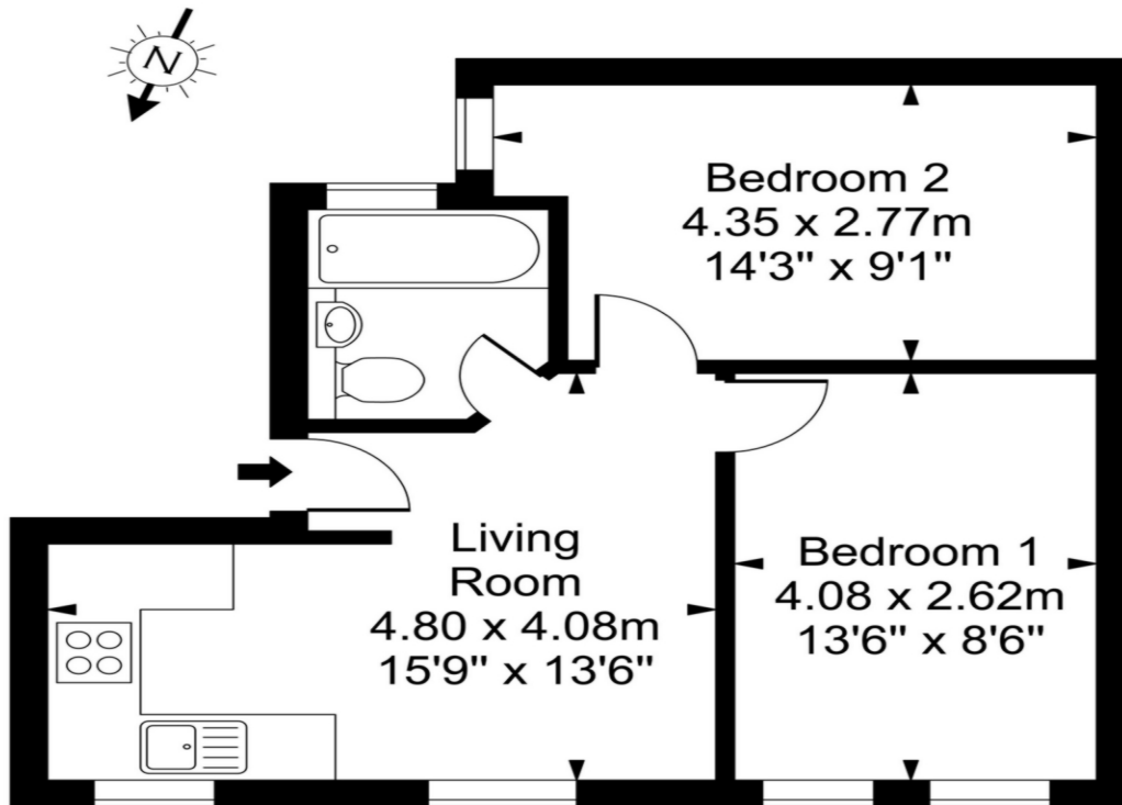
Second Floor
